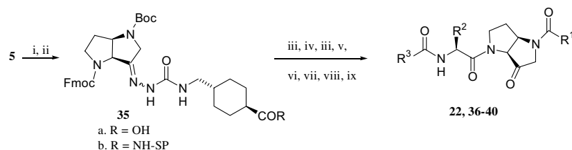
Scheme 5. Synthesis and use of supported linker construct 35b towards full length inhibitors 22 , 36–40 . Reagents and conditions: (i) trans -4{[(hydrazinocarbonyl) amino]methyl}cyclohexanecarboxylic acid trifluoroacetate, 18 EtOH, H 2 O, NaOAc, reflux; (ii) 3equiv 35a , 3equiv HBTU, 3equiv HOBt, 6equiv NMM, H 2 N-SOLID PHASE, DMF; (iii) 20% piperidine/DMF (v/v), 30min; (iv) 20equiv Fmoc-NHCHR 2 -COOH, 20equiv HBTU, 20equiv HOBt, 40equiv NMM, DMF, rt, o/n, then repeat with fresh reagents for 6h; (v) 10equiv R 3 -COOH, 10equiv HBTU, 10equiv HOBt, 20equiv NMM, DMF, rt o/n; (vi) TFA/DCM (35:65, v/v), 30min; (vii) NMM/DMF (2:98, v/v), 10min; (viii) 20equiv benzoic anhydride, 10equiv NMM, DMF, o/n; (ix) TFA/H 2 O, (95:5, v/v), 2h.
