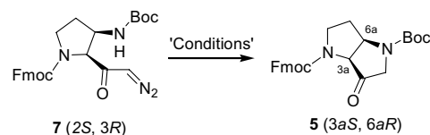
Scheme 1. Synthesis of (3aS,6aR)-5 via an N–H insertion reaction of (3R)- tert -butoxycarbonylamino-(2S)-(2-diazoacetyl)pyrrolidine-1-carboxylic acid 9H-fluoren-9-ylmethyl ester.
