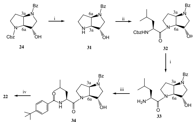
Scheme 4. Solution synthesis of (3a R ,6a S )- 22 via alcohol. Reagents and conditions: (i) Pd–C/H 2 , ethanol/methanol; (ii) 1 equiv Cbz-Leu-F, DMF, rt; (iii) 1 equiv 4- tert -butylbenzoic acid, HBTU, HOBT, NMM, DMF, rt; (iv) Dess–Martin periodinane, DCM, 2 equiv TFA.
