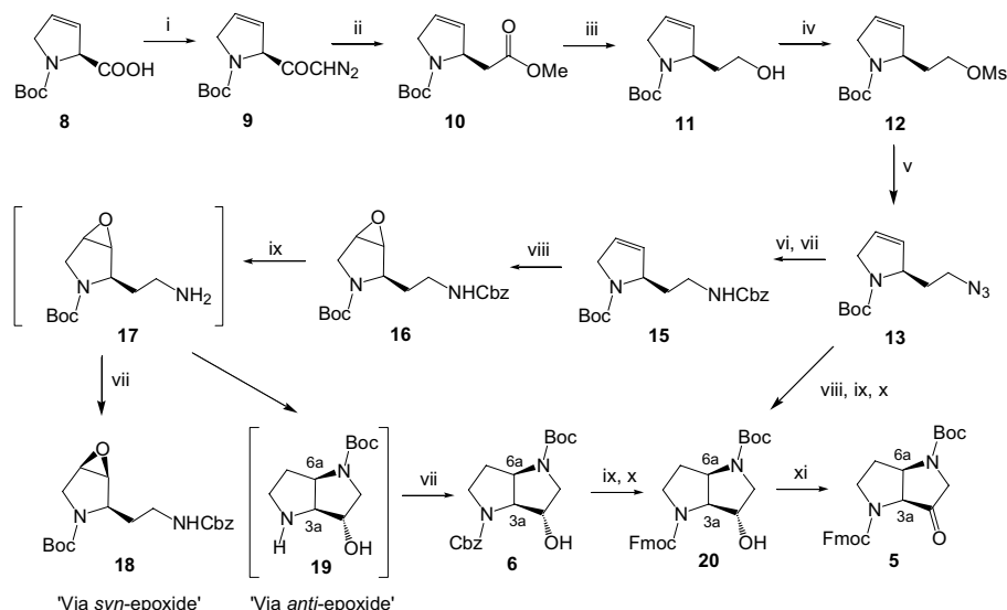
Scheme 2. Synthesis of (3a S ,6a R )- 5 and 6 . Reagents and conditions: (i) (a) isobutyl chloroformate, NMM, CH 2 Cl 2 , –15°C; (b) ethereal CH 2 N 2 , –15°C to rt; (ii) MeOH, THF, CF 3 CO 2 Ag, NMM, 0°C to rt in dark; (iii) LiBH 4 , MeOH, THF; (iv) methanesulfonyl chloride, triethylamine, DCM; (v) sodium azide, DMF; (vi) Ph 3 P, H 2 O, THF; (vii) 1.05 equiv Cbz–Cl, 2.1 equiv Na 2 CO 3 , 1,4-dioxane, water; (viii) m -chloroperoxybenzoic acid, DCM, rt, o/n; (ix) Pd–C/H 2 , ethanol; (x) 1.05 equiv Fmoc–Cl, 2.1 equiv Na 2 CO 3 , 1,4-dioxane, water; (xi) Dess–Martin periodinane, DCM.
