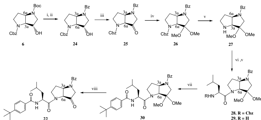
Scheme 3. Solution synthesis of (3a R ,6a S )- 22 via ketal. Reagents and conditions: (i) 4 N HCl in 1,4-dioxane, 30 min, rt; (ii) benzoic anhydride, NMM, DMF, rt, 1 h; (iii) Dess–Martin periodinane, DCM; (iv) trimethylorthoformate, anhydrous MeOH, cat. p -TsOH, under Ar, 65 °C; (v) Pd–C/H 2 , ethanol, methanol; (vi) 1 equiv Cbz-Leu-F, DMF, rt; (vii) 1 equiv 4- tert -butylbenzoic acid, HBTU, HOBT, NMM, DMF, rt; (viii) 95% TFA/5% water, rt.
